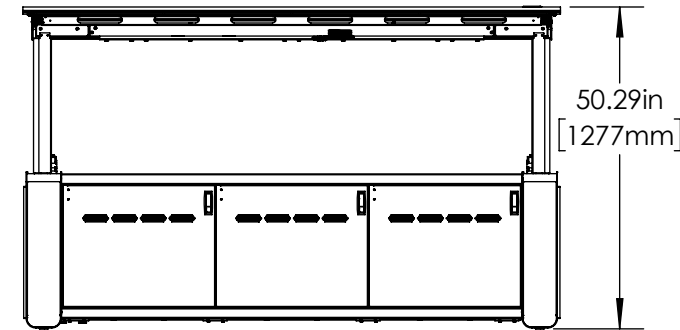
Pinnacle 84" Front View-Standing
