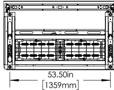
Pinnacle 60" Bottom View
