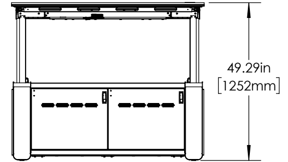
Pinnacle 60" Front View-Standing
