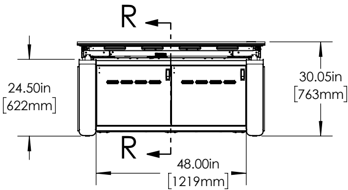
Pinnacle 60" Front View-Sitting
