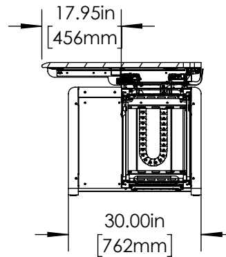
Pinnacle 60" Side View-Sitting
