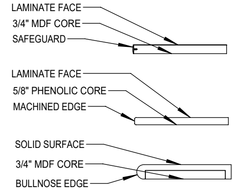
6 Work Surface Edge Types Typical
