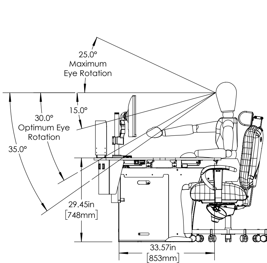
① Vue P Open Base Dual Sit-Stand Ergonomic Detail - Sitting
