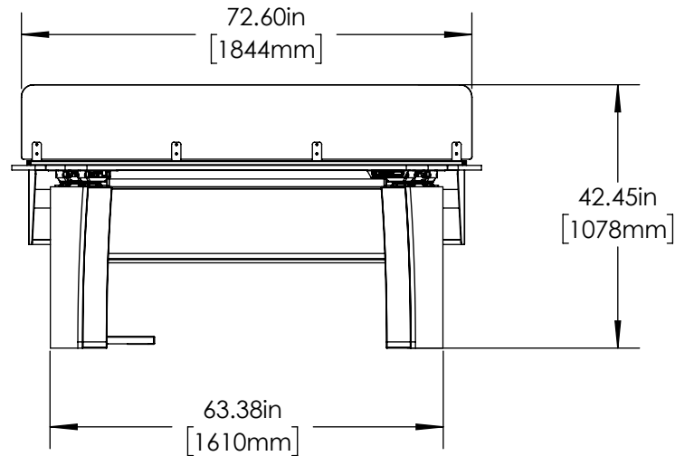
③ Vue P Open Base Dual Sit-Stand Front
