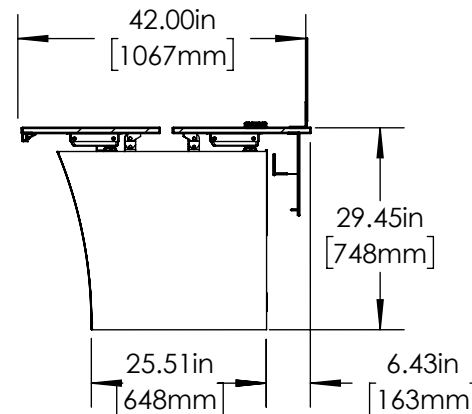
④ Section T-T - Vue P Open Base Dual Sit-Stand Side
