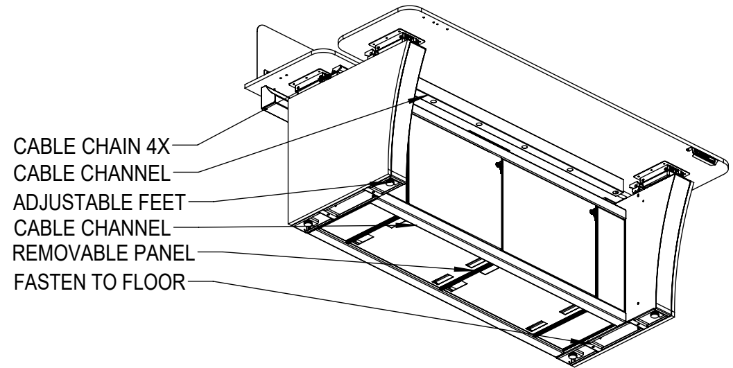
③ Vue X Closed Base Dual Sit/Stand ISO-Bottom
