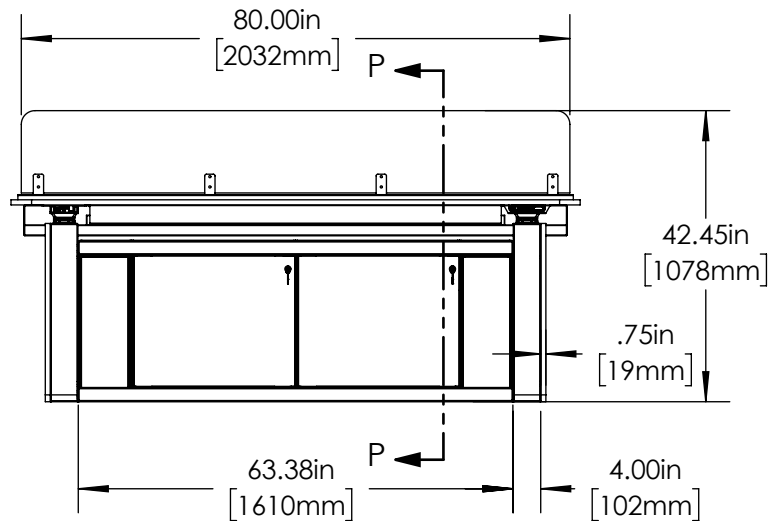
③ Vue X Closed Base Dual Sit/Stand Front
