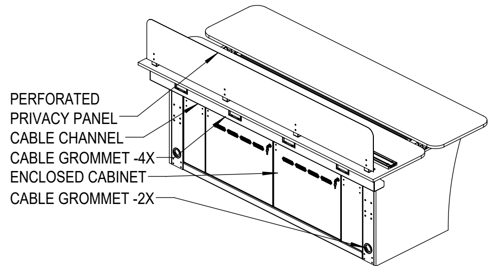
② Vue X Closed Base Dual Sit/Stand ISO-Back
