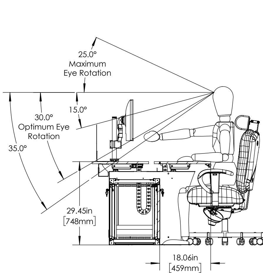
① Vue X Closed Base Dual Sit/Stand Ergonomic Detail - Sitting
