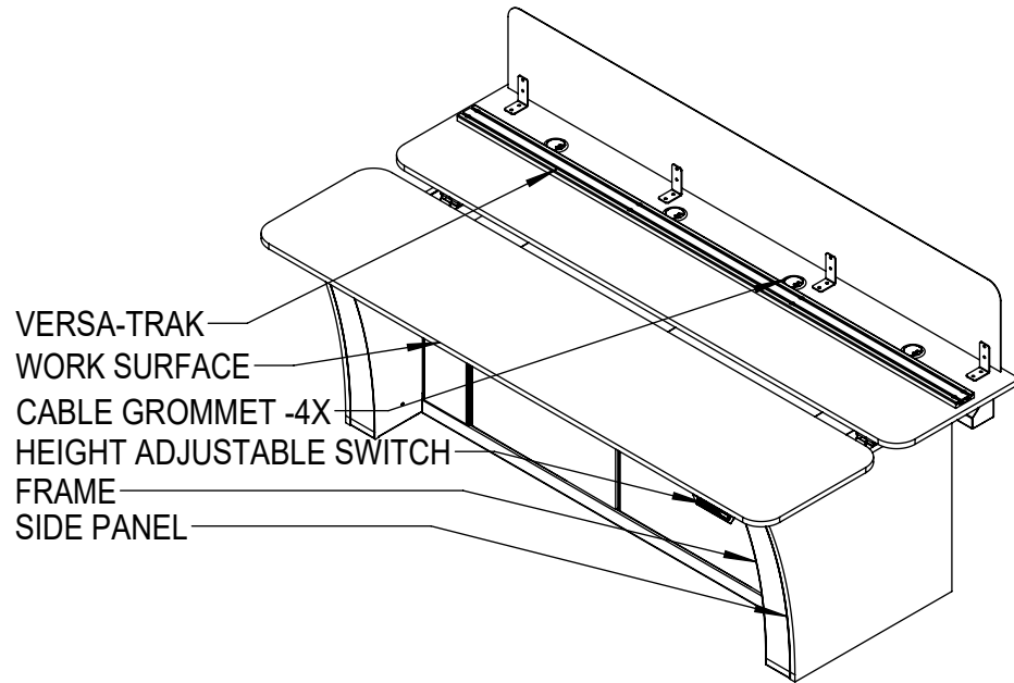
① Vue X Closed Base Dual Sit/Stand ISO-Front
