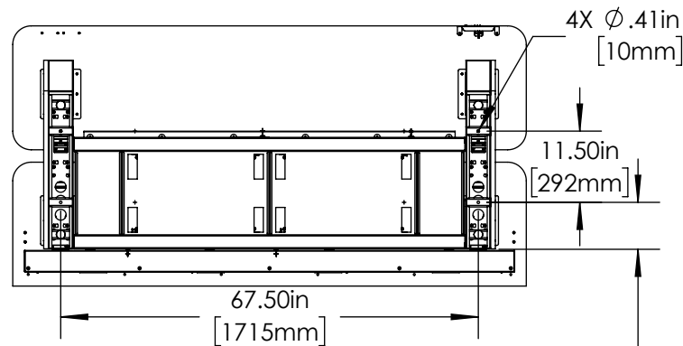
② Vue X Closed Base Dual Sit/Stand Bottom
