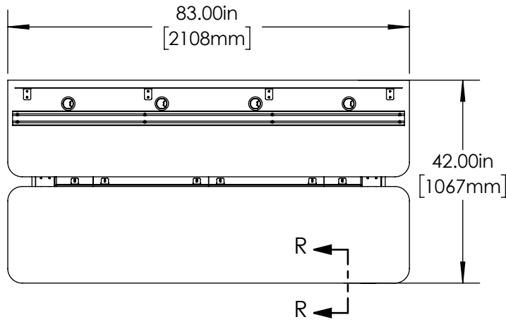
① Vue X Closed Base Dual Sit/Stand Top
