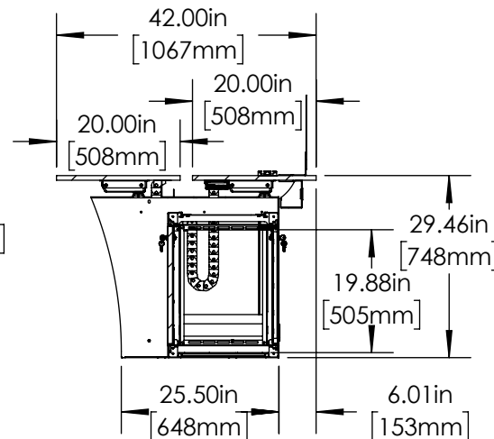
② Vue X Closed Base Dual Sit/Stand Bottom
