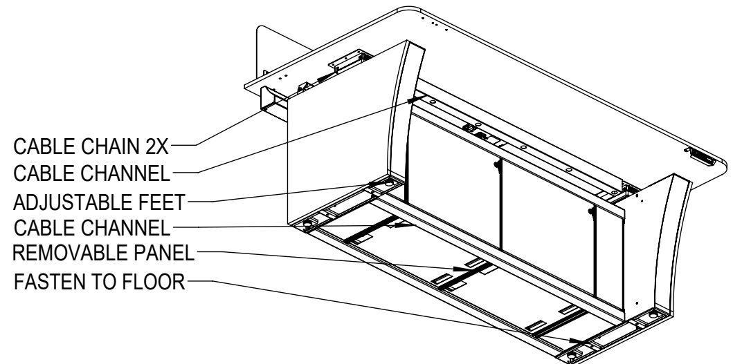
③ Vue X Closed Base Sit/Stand ISO-Bottom
