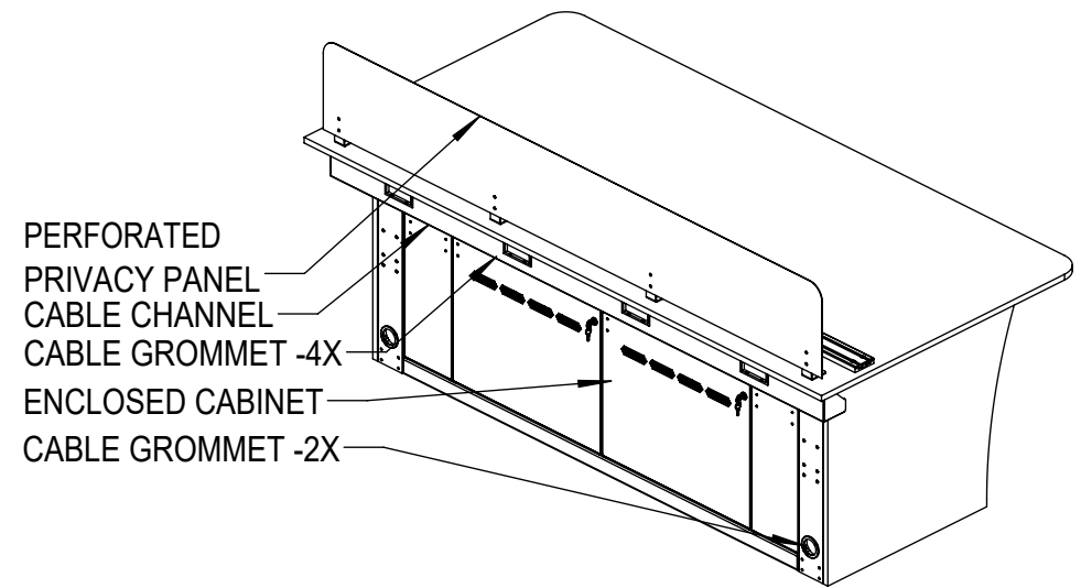
② Vue X Closed Base Sit/Stand ISO-Back
