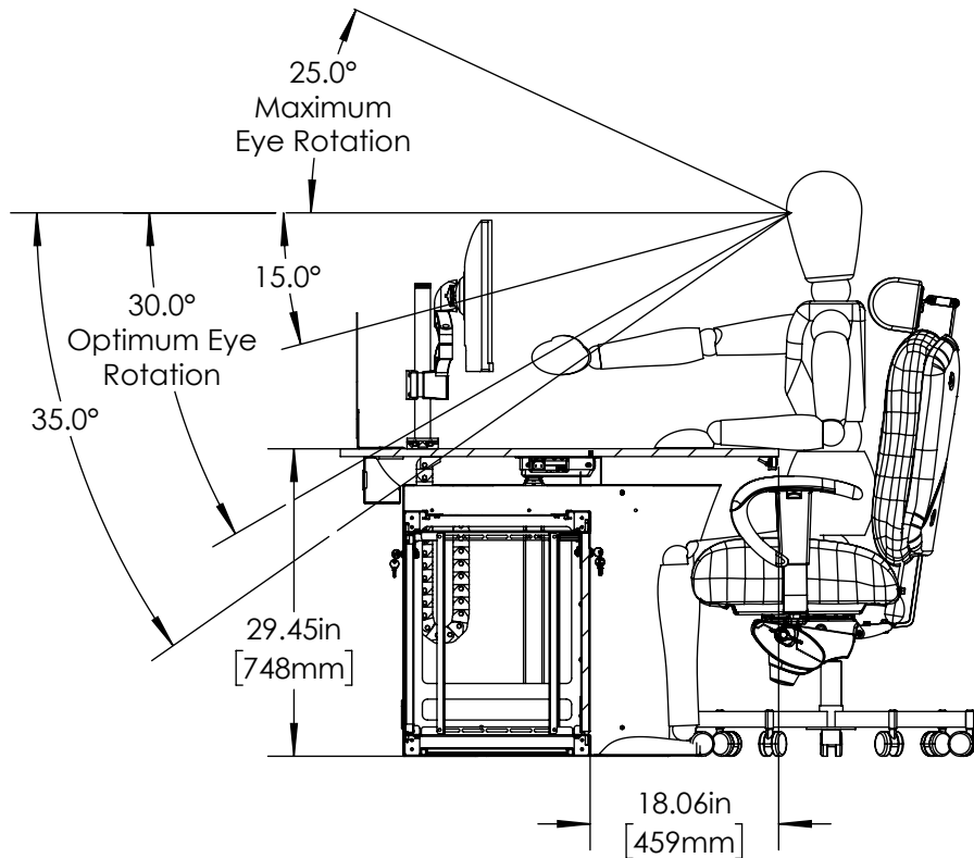
① Vue X Closed Base Sit/Stand Ergonomic Detail - Sitting
