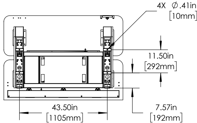
② Vue L Closed Base Dual Sit/Stand Bottom
