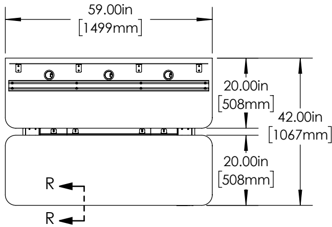
① Vue L Closed Base Dual Sit/Stand Top
