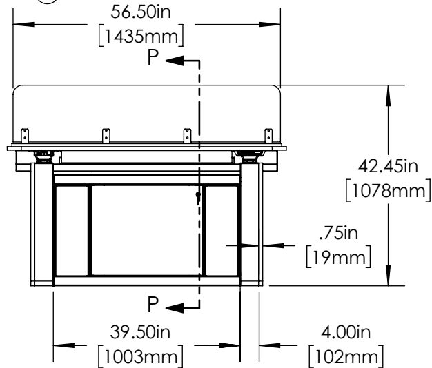
③ Vue L Closed Base Dual Sit/Stand Front
