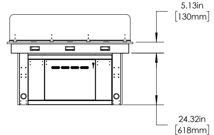
⑤ Vue L Closed Base Dual Sit/Stand Back
