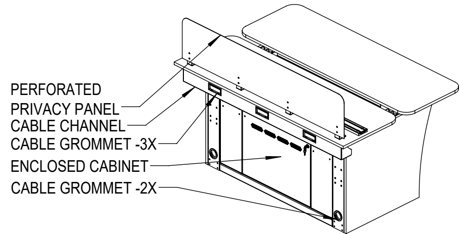
② Vue L Closed Base Sit/Stand ISO-Back
