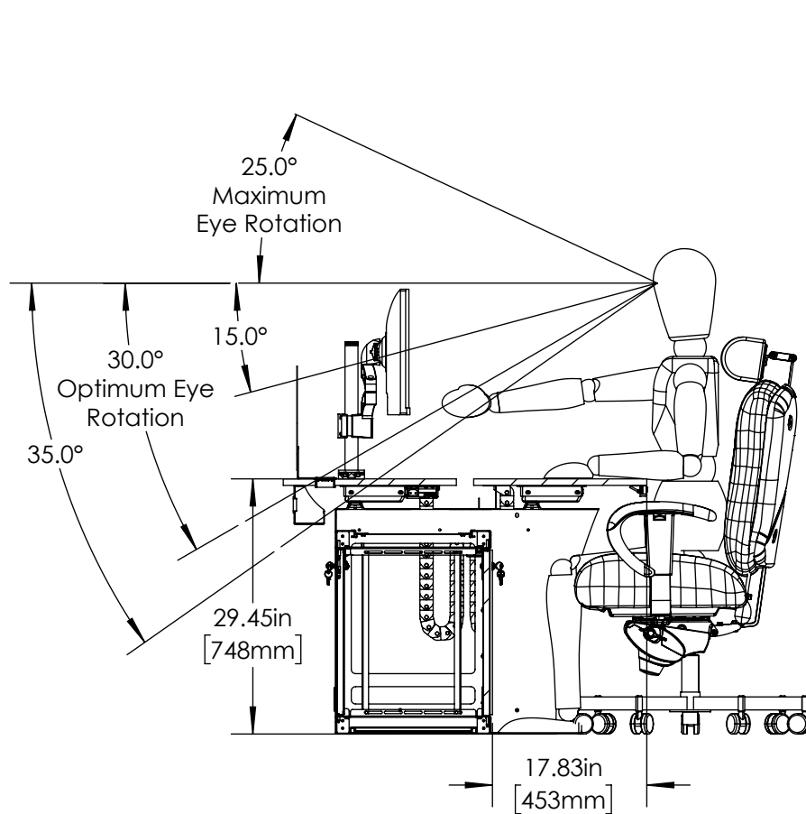
① Vue L Closed Base Dual Sit/Stand Ergonomic Detail - Sitting
