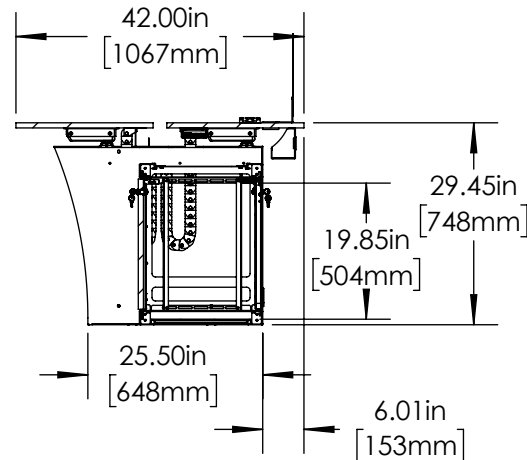
④ Section P-P - Vue L Closed Base Dual Sit/Stand Side
