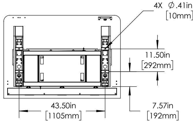
② Vue L Closed Base Sit/Stand Bottom
