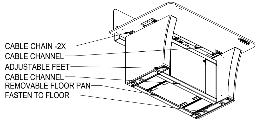
③ Vue L Closed Base Sit/Stand ISO-Bottom
