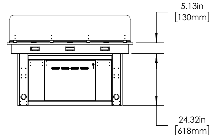
⑤ Vue L Closed Base Sit/Stand Back
