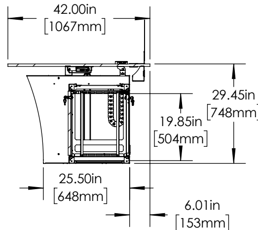
④ Section P-P - Vue L Closed Base Sit/Stand Side
