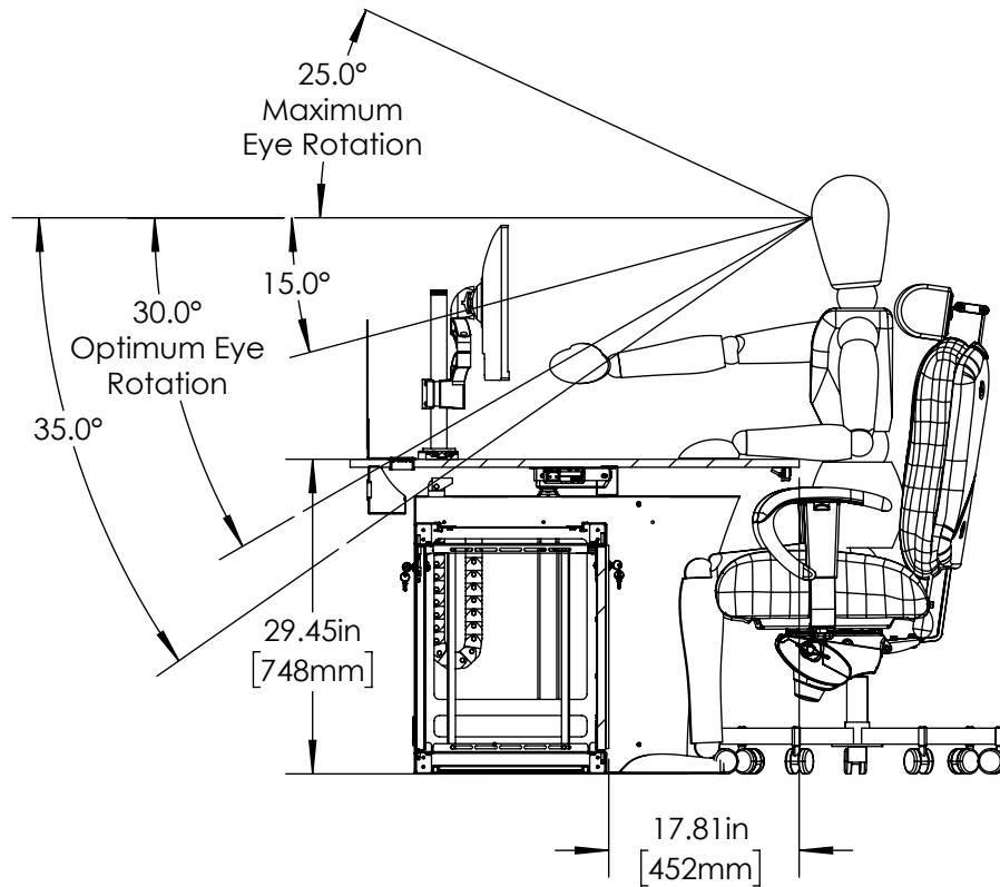
① Vue L Closed Base Sit/Stand Ergonomic Detail - Sitting
