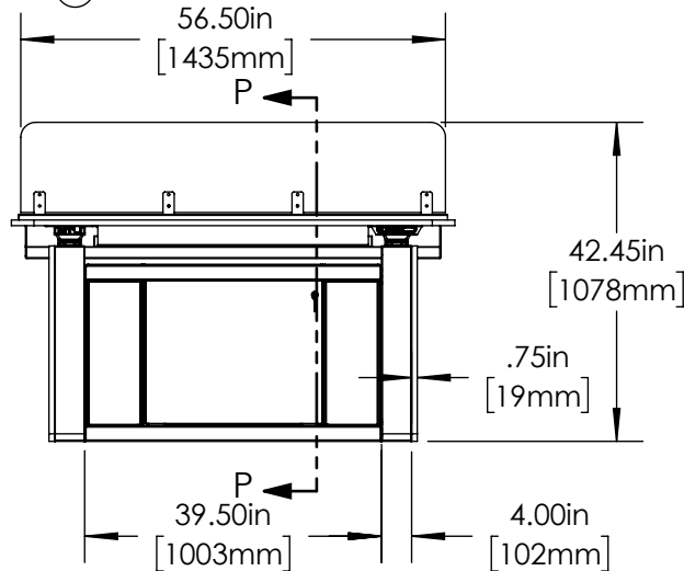
① Vue L Closed Base Sit/Stand Top
