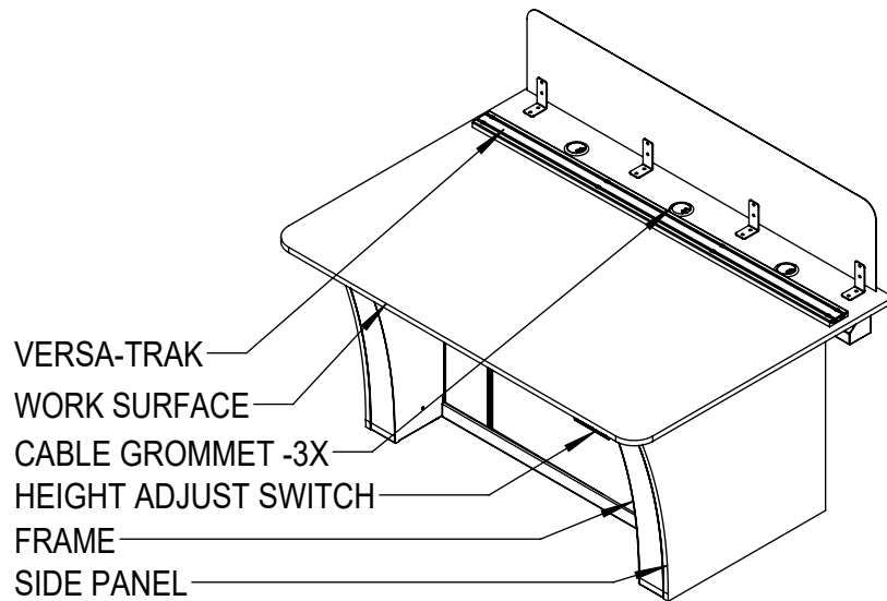
① Vue L Closed Base Sit/Stand ISO-Front
